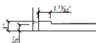
Section at Threshold
